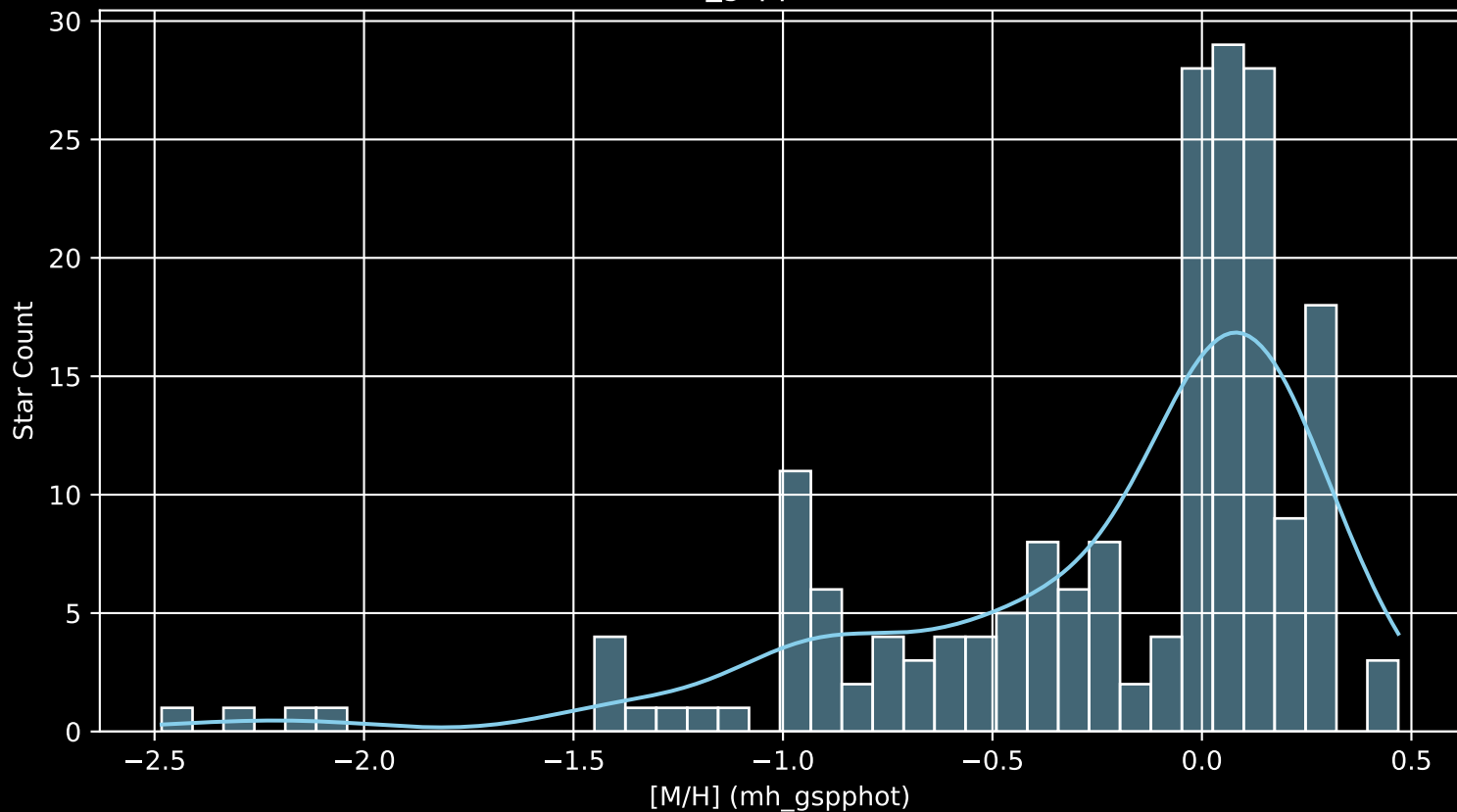
APOGEE DR17 Field: [135-03 [M/H] (mh_gspphot) (n= 194)
