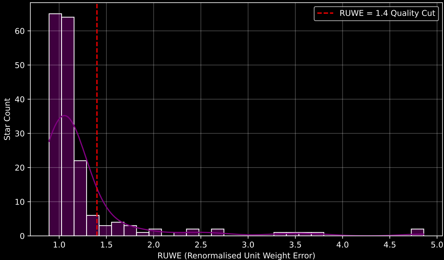
GAPOGEE DR17 Field [135-03] RUWE Distribution (n= 181)
