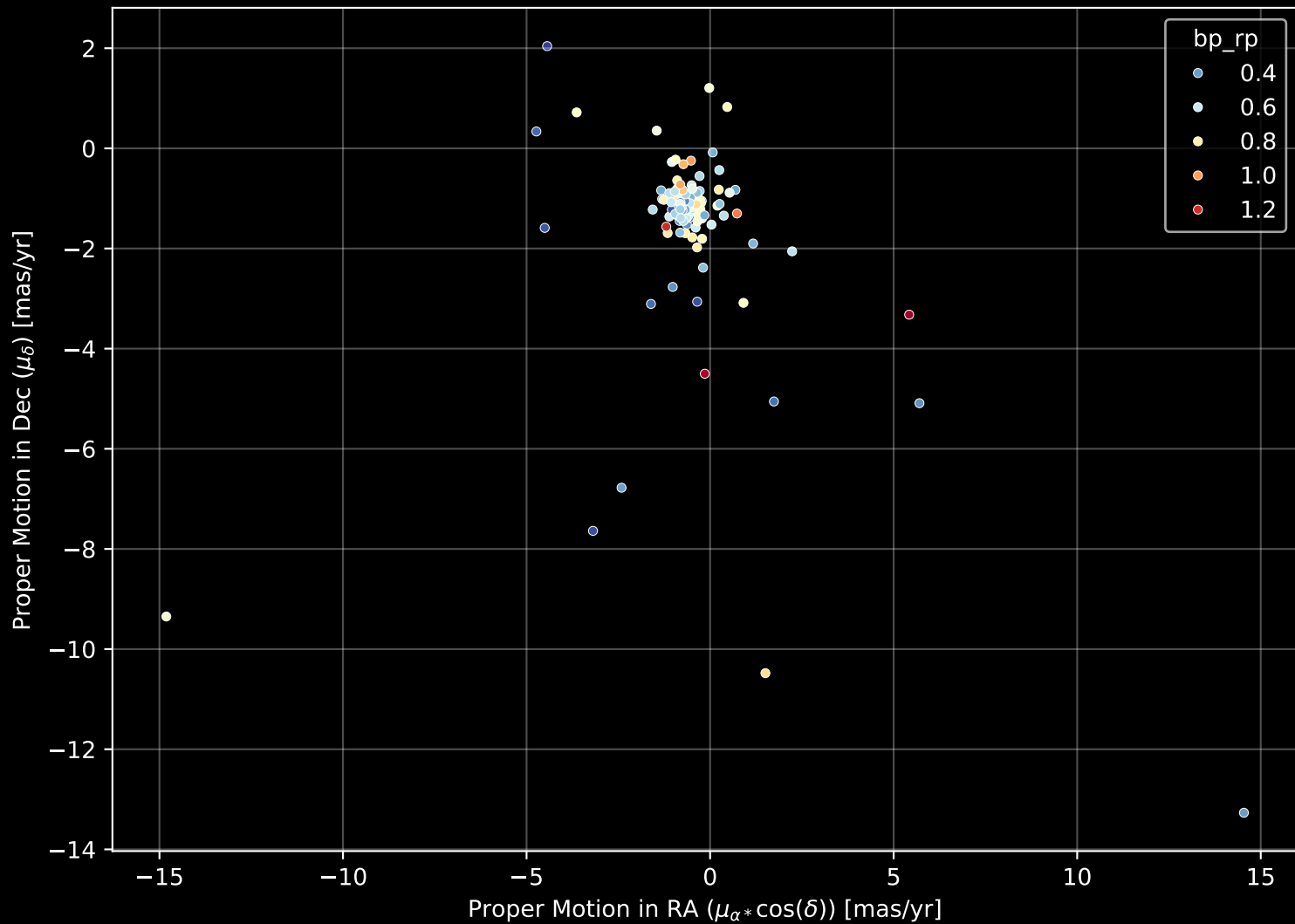
APOGEE DR17 Field: [135-03] Proper Motion Diagram (n= 195)
