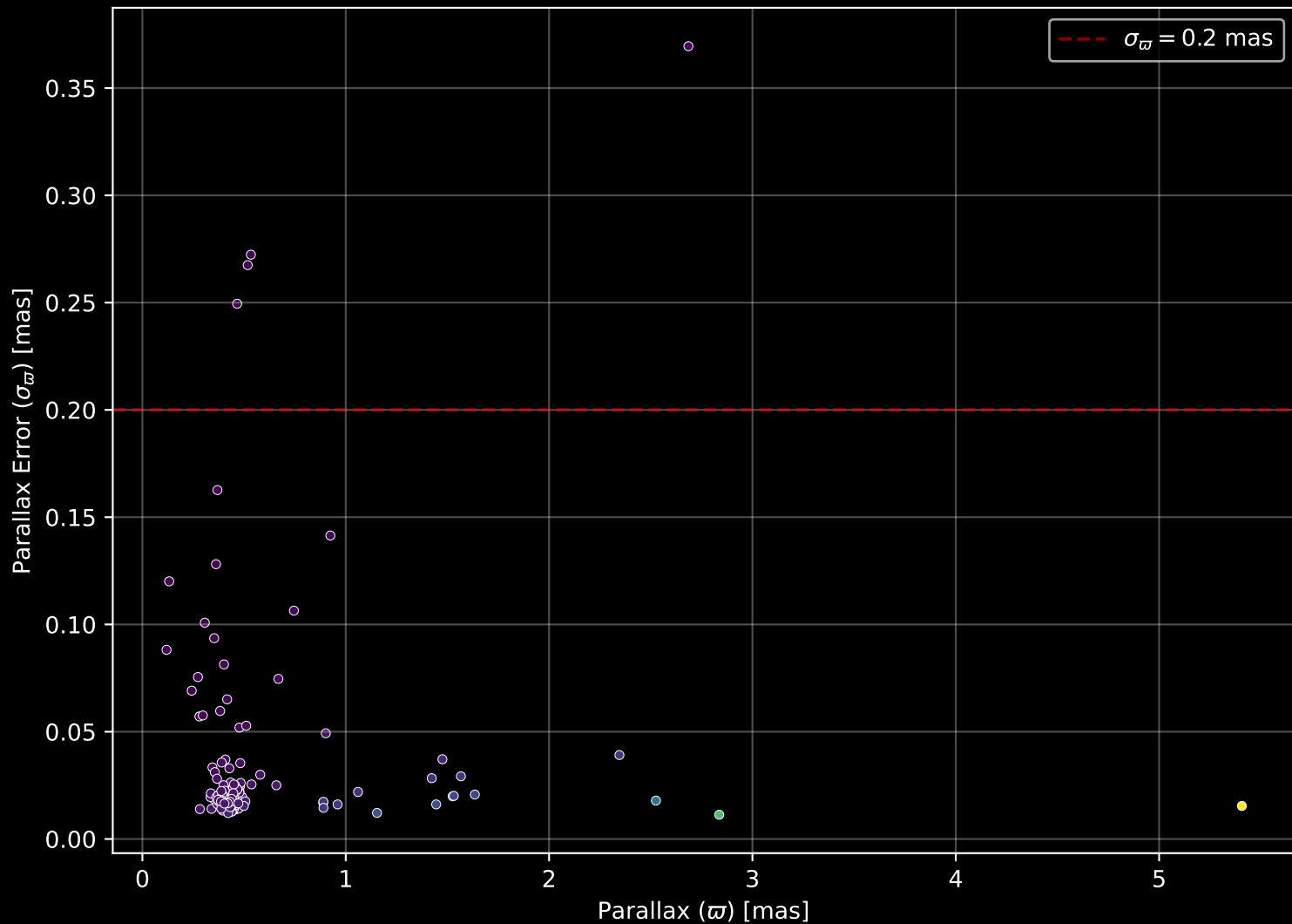
APOGEE DR17 Field: [135-03] Parallax Quality (n= 195)
