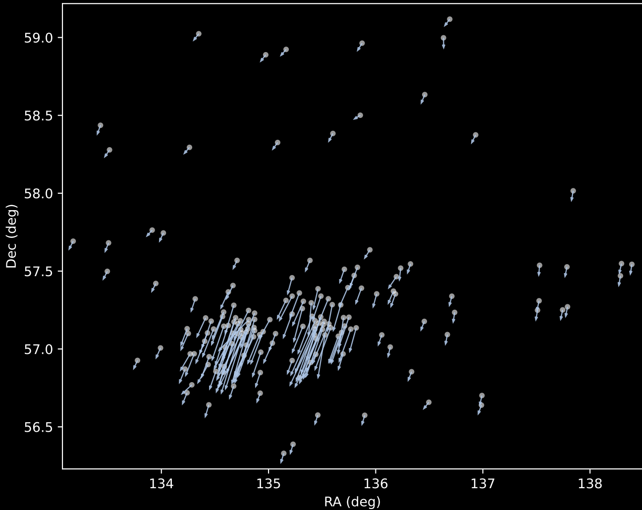
APOGEE DR17 Cluster 1 Proper Motion Vectors (n=158)
