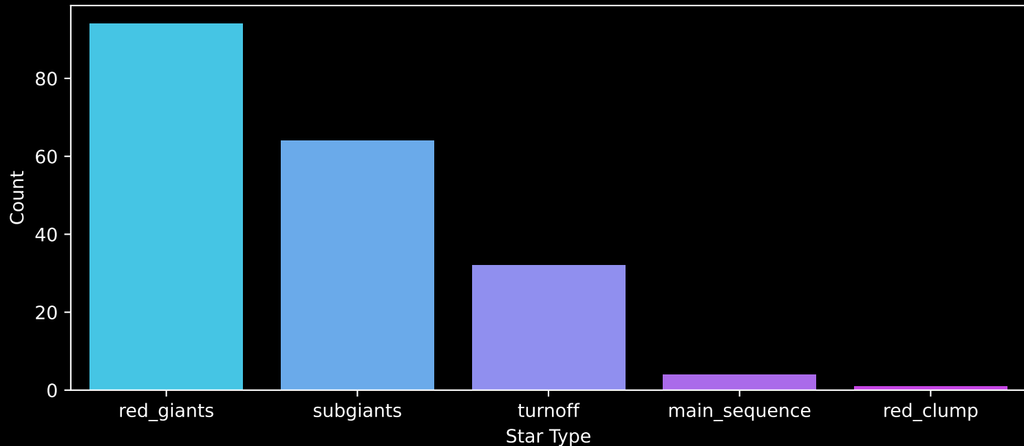
APOGEE DR17 Field: [135-03] Count plot of Star Type
