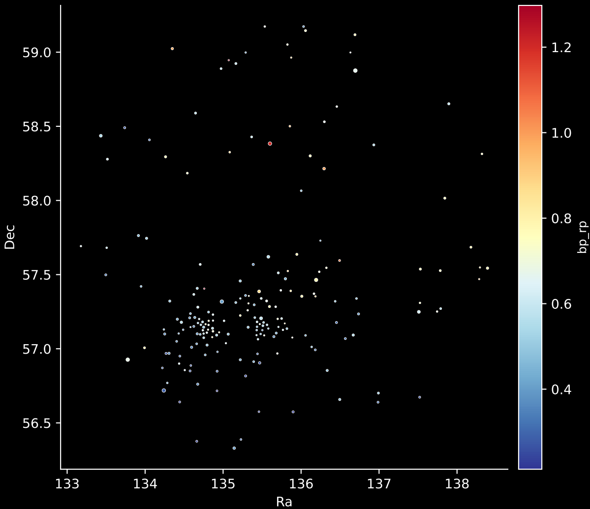
APOGEE DR17 Field: [135-03] Stars: 195
